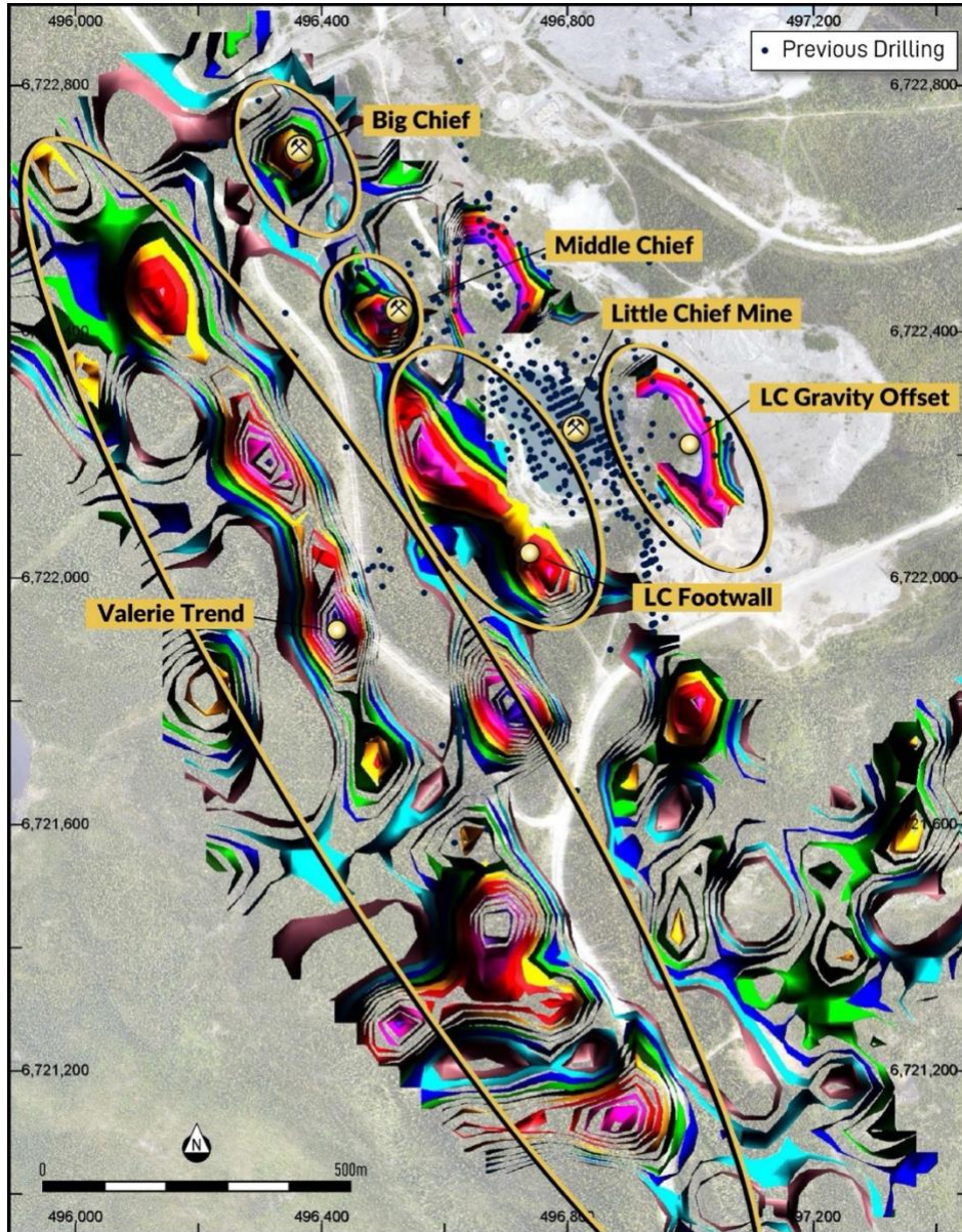
Figure 1: Plan map of the Little Chief Trend with copper-gold skarn targets identified and highlighted over contoured gravimetric survey and regional drone-borne aeromagnetic.
